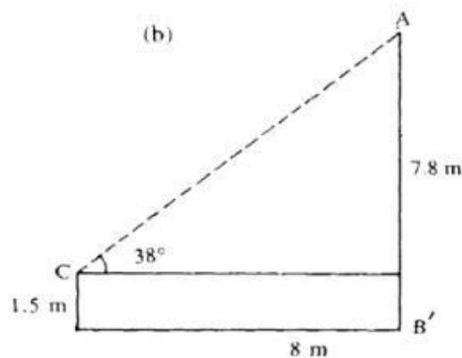
Scale drawing
